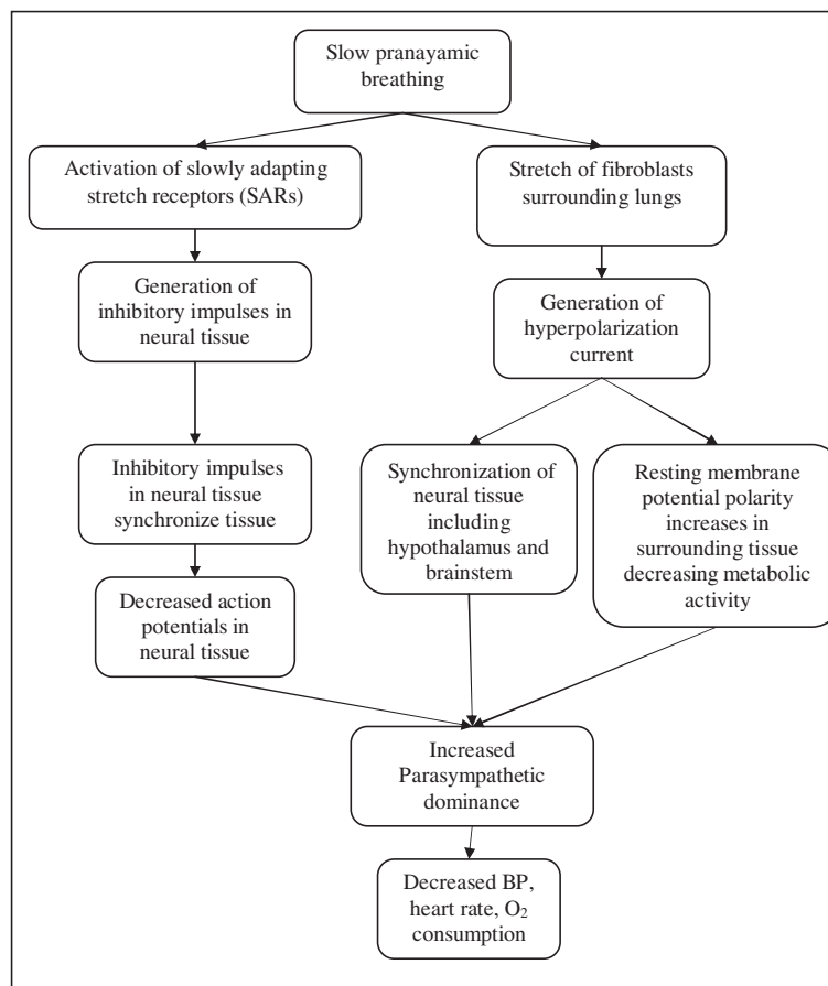
Figure 1 Diagram of the series of events that occur during the autonomic shift present in pranayamic slow breathing.
